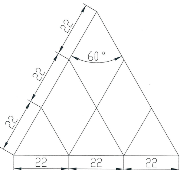
DETAIL DRAWING OF TUBE PITCH 孔距详图 1:1
